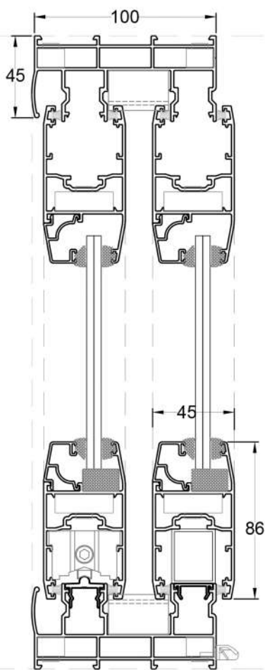
Corte Vertical
